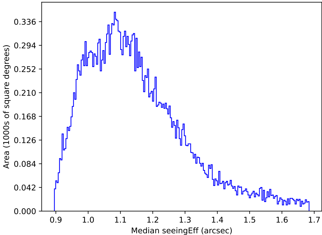
ddf_acor_sf30_lsf40_lsr10_v3.4_10yrs All sky g band: Median seeingEff
