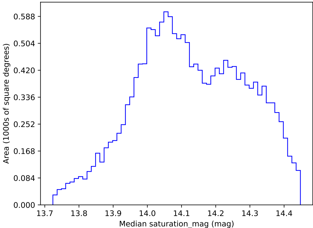
ddf_acor_sf30_lsf40_lsr10_v3.4_10yrs WFD z band: Median saturation_mag
