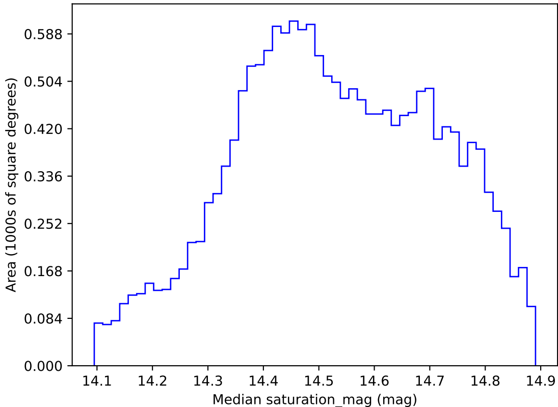
ddf_acor_sf30_lsf40_lsr10_v3.4_10yrs WFD i band: Median saturation_mag
