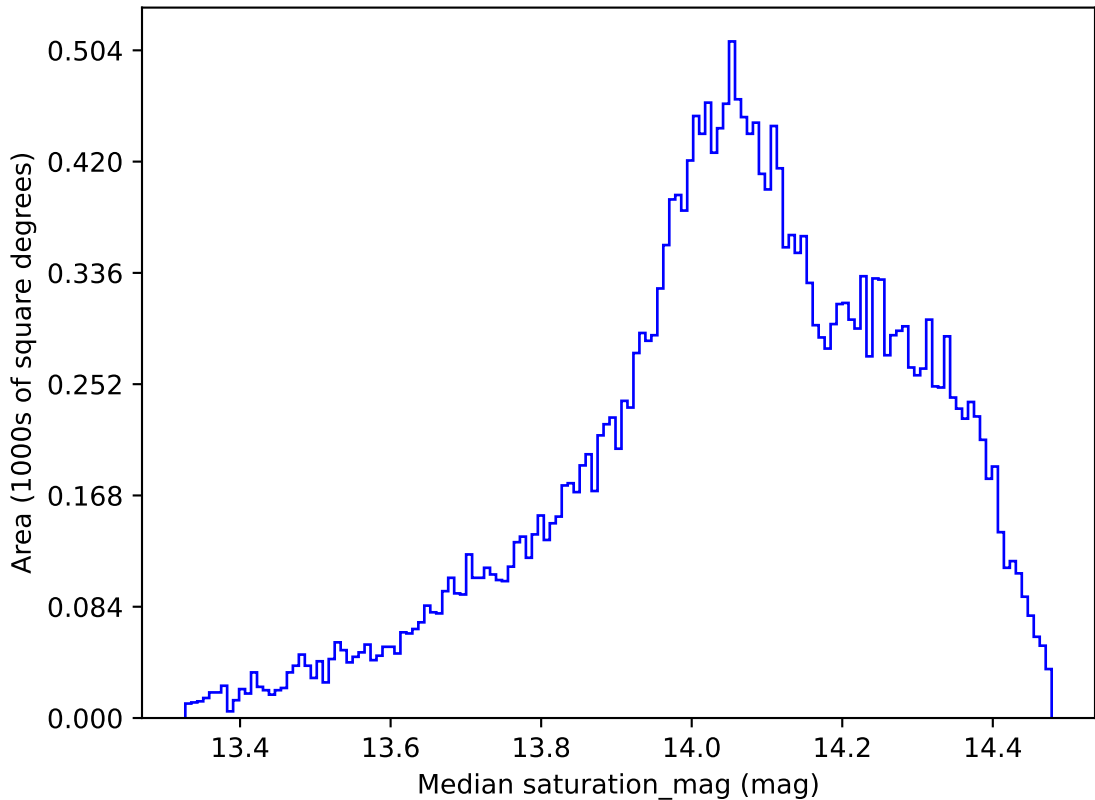
ddf_acor_sf30_lsf40_lsr10_v3.4_10yrs All sky z band: Median saturation_mag
