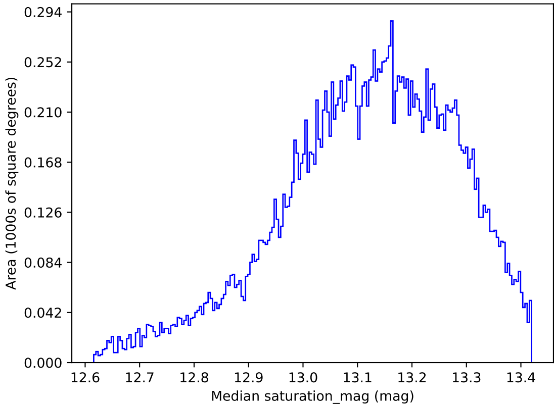
ddf_acor_sf30_lsf40_lsr10_v3.4_10yrs All sky y band: Median saturation_mag
