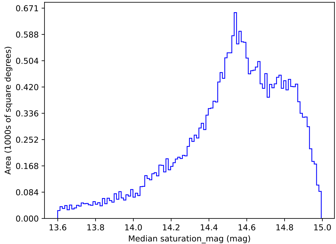
ddf_acor_sf30_lsf40_lsr10_v3.4_10yrs All sky r band: Median saturation_mag
