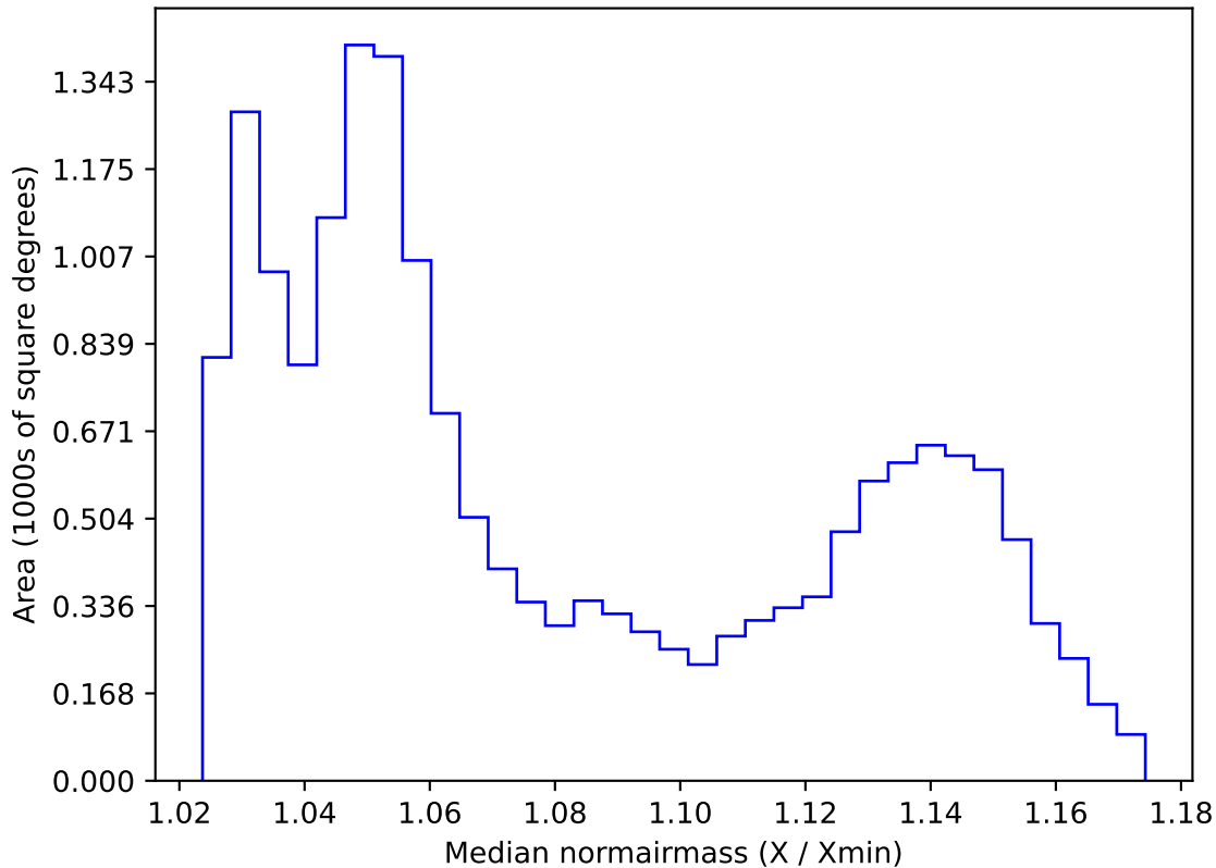
ddf_acor_sf30_lsf40_lsr10_v3.4_10yrs WFD all bands: Median normairmass
