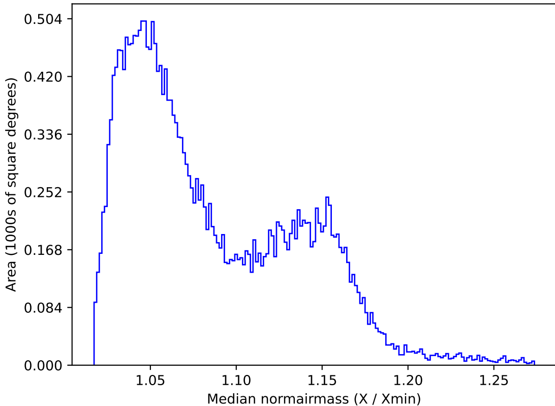
ddf_acor_sf30_lsf40_lsr10_v3.4_10yrs All sky z band: Median normairmass
