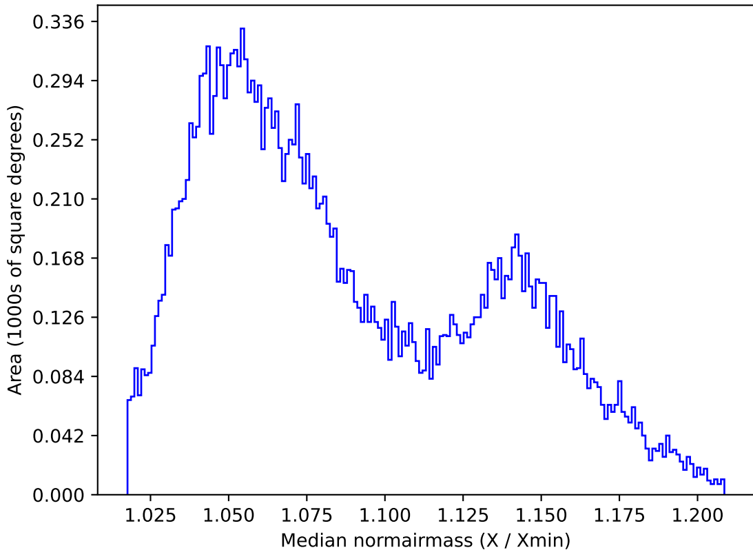
ddf_acor_sf30_ls40_lsr10_v3.4_10yrs All sky y band: Median normairmass
