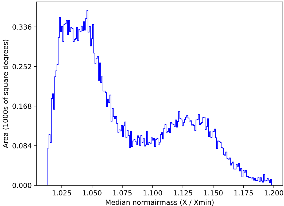
ddf_acor_sf30_lsf40_lsr10_v3.4_10yrs All sky r band: Median normairmass
