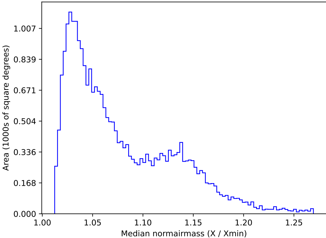
ddf_acor_sf30_lsf40_lsr10_v3.4_10yrs All sky g band: Median normairmass
