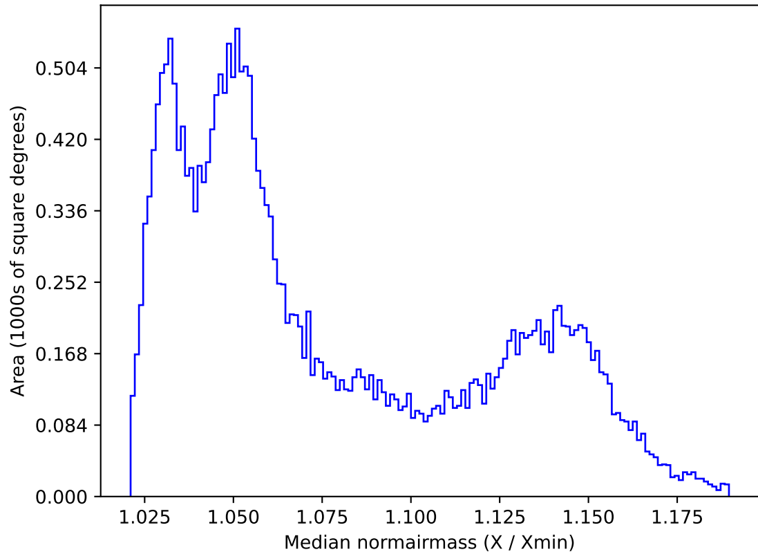
ddf_acor_sf30_lsf40_lsr10_v3.4_10yrs All sky all bands: Median normairmass
