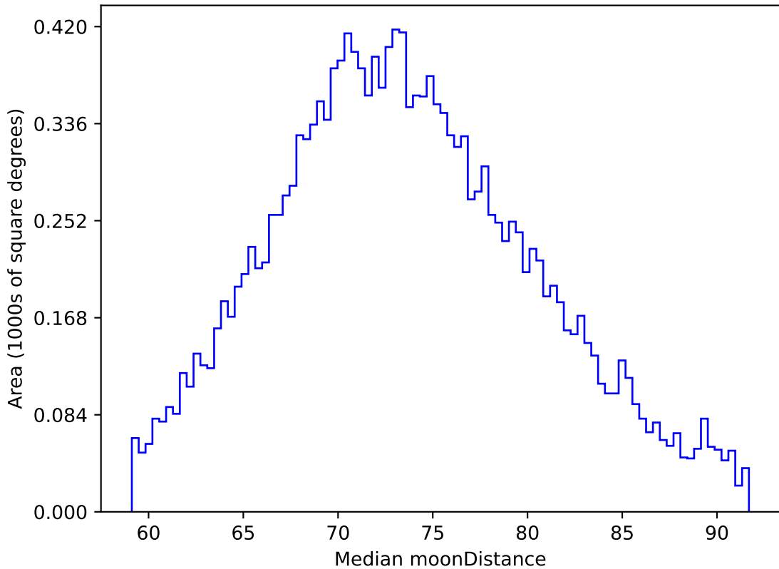
ddf_acor_sf30_lsf40_lsr10_v3.4_10yrs WFD z band: Median moonDistance
