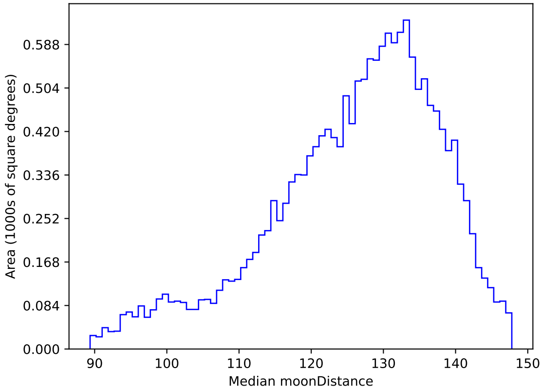
ddf_acor_sf30_ls40_lsr10_v3.4_10yrs WFD u band: Median moonDistance
