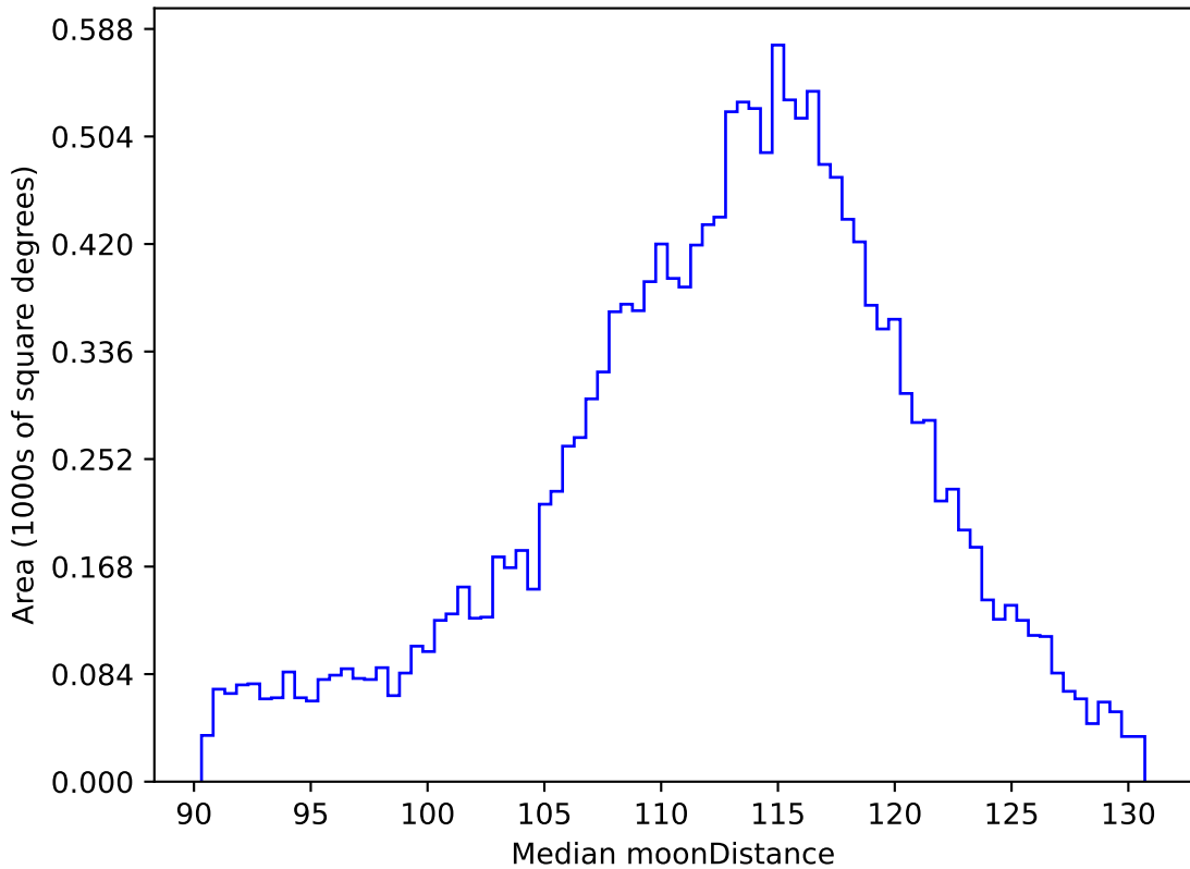
ddf_acor_sf30_lsf40_lsr10_v3.4_10yrs WFD r band: Median moonDistance
