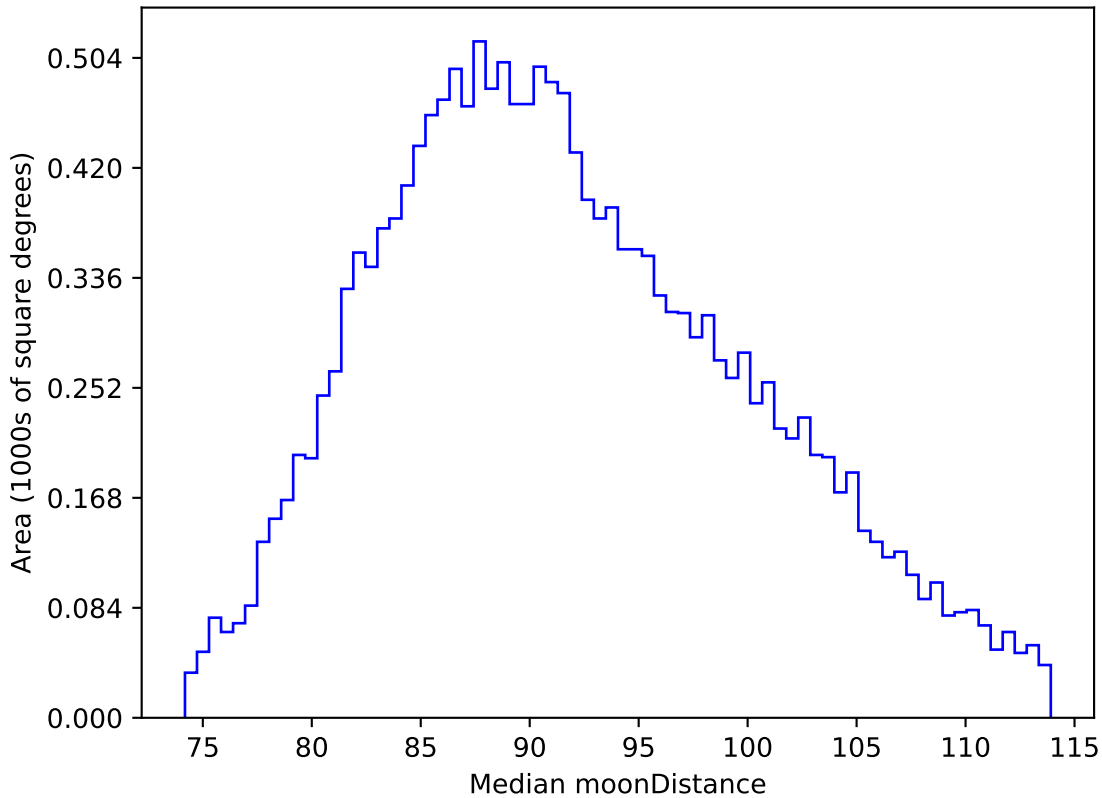
ddf_acor_sf30_lsf40_lsr10_v3.4_10yrs WFD i band: Median moonDistance
