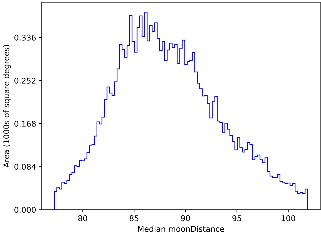
ddf_acor_sf30_lsf40_lsr10_v3.4_10yrs WFD all bands: Median moonDistance
