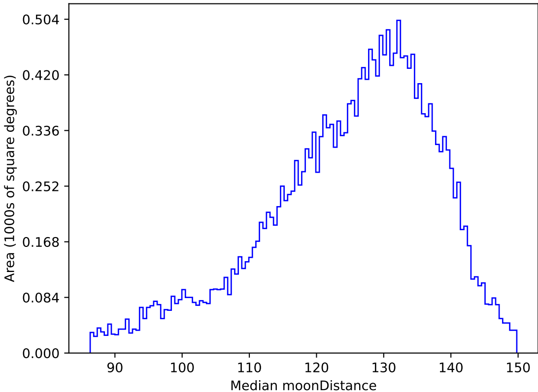
ddf_acor_sf30_lsf40_lsr10_v3.4_10yrs All sky u band: Median moonDistance
