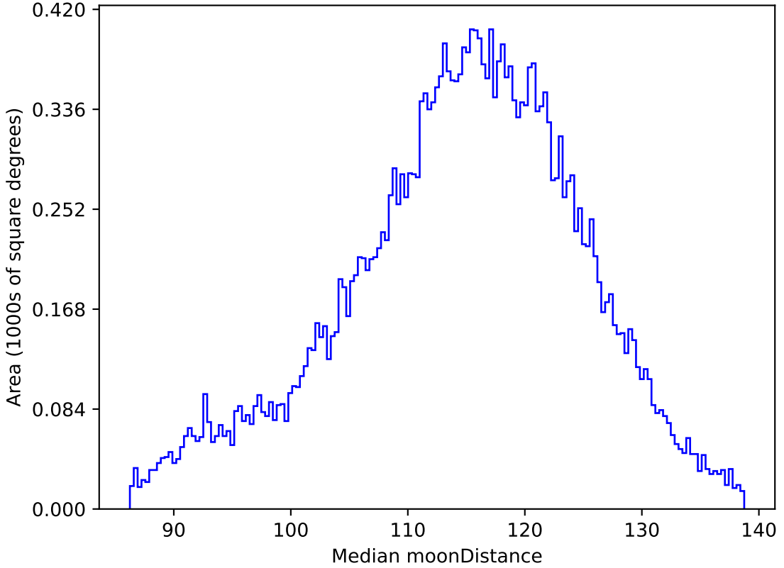
ddf_acor_sf30_lsf40_lsr10_v3.4_10yrs All sky g band: Median moonDistance
