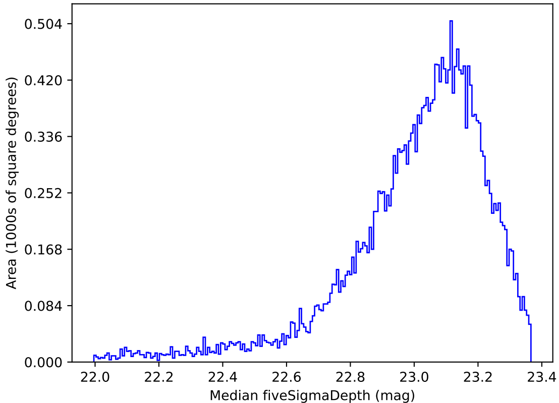
ddf_acor_sf30_lsf40_lsr10_v3.4_10yrs Yr 1 z band: Median fiveSigmaDepth
