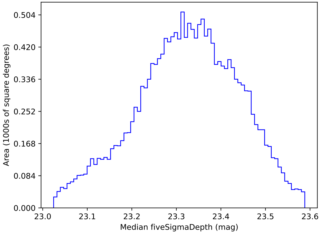
ddf_acor_sf30_lsf40_lsr10_v3.4_10yrs WFD all bands: Median fiveSigmaDepth
