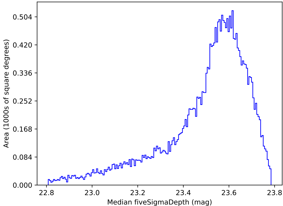
ddf_acor_sf30_lsf40_lsr10_v3.4_10yrs All sky i band: Median fiveSigmaDepth
