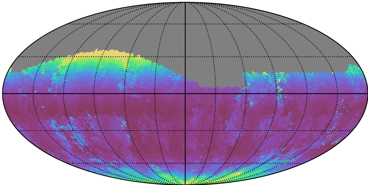
ddf_acor_sf30_lsf40_lsr10_v3.4_10yrs Yr 1 g band: Median airmass
