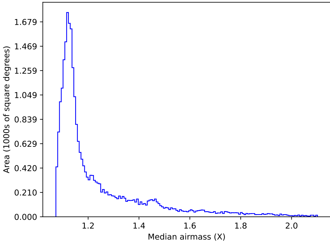
ddf_acor_sf30_lsf40_lsr10_v3.4_10yrs Yr 1 all bands: Median airmass
