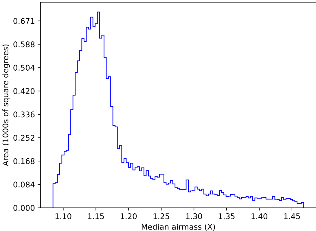
ddf_acor_sf30_lsf40_lsr10_v3.4_10yrs WFD z band: Median airmass
