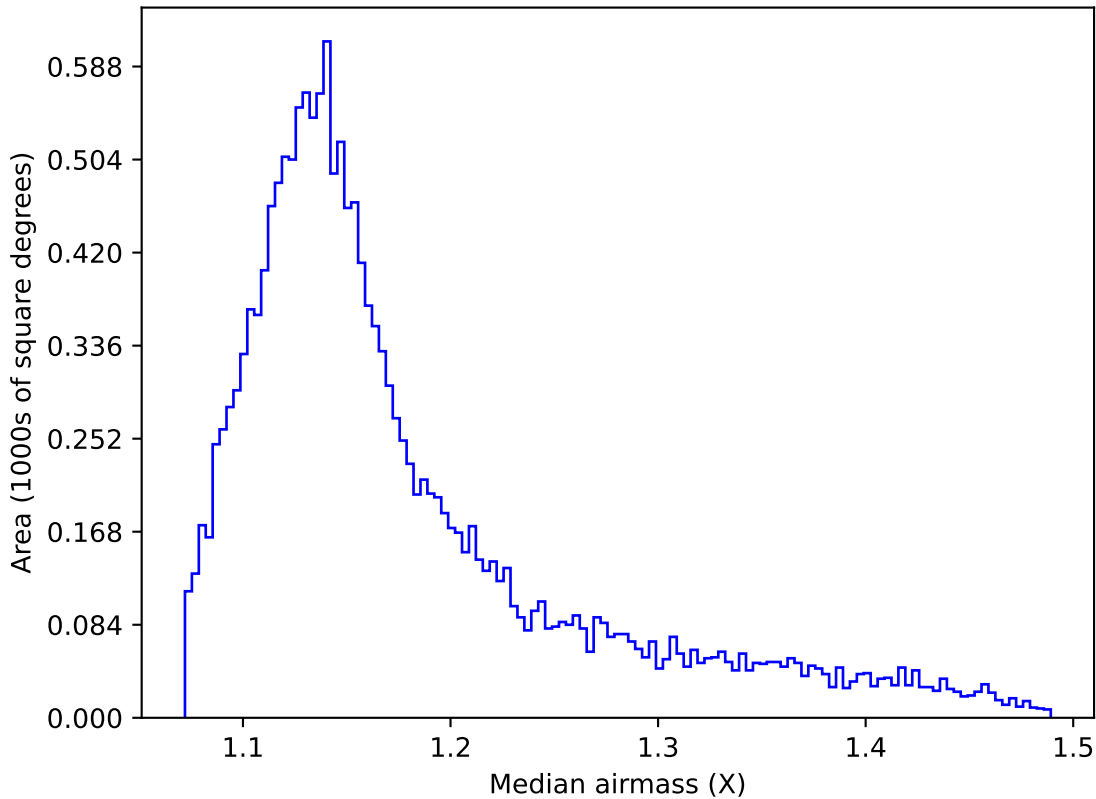
ddf_acor_sf30_ls40_lsr10_v3.4_10yrs WFD g band: Median airmass
