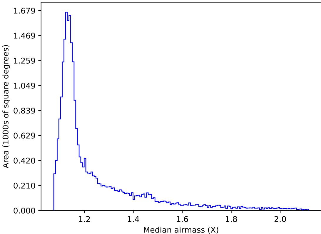
ddf_acor_sf30_lsf40_lsr10_v3.4_10yrs All sky r band: Median airmass
