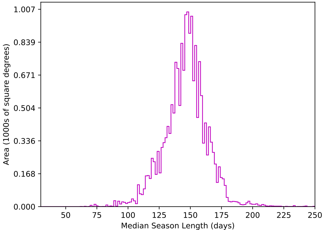
ddf_acor_sf30_lsf40_lsr10_v3.4_10yrs WFD z band: Median Season Length
