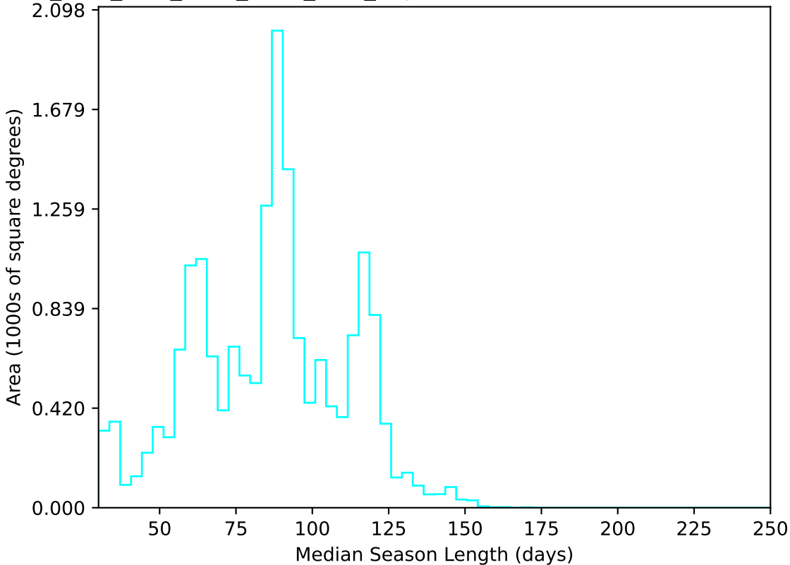
ddf_acor_sf30_ls40_lsr10_v3.4_10yrs WFD u band: Median Season Length
