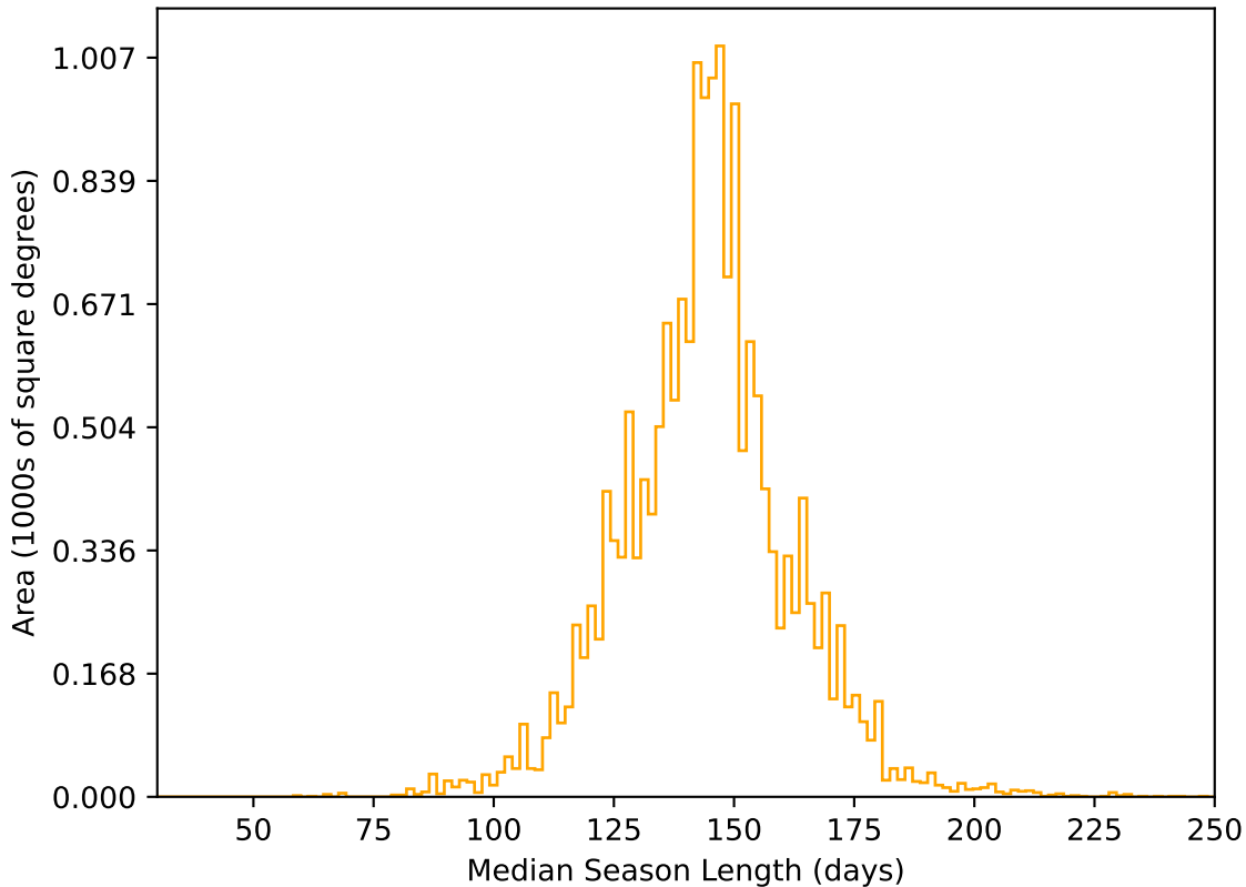
ddf_acor_sf30_lsf40_lsr10_v3.4_10yrs WFD r band: Median Season Length
