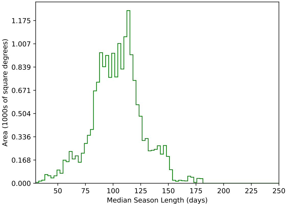
ddf_acor_sf30_lsf40_lsr10_v3.4_10yrs WFD g band: Median Season Length
