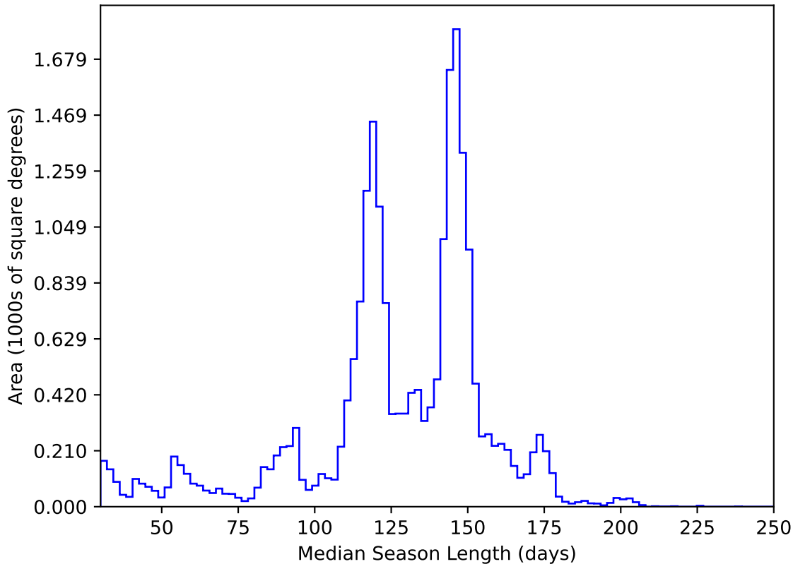
ddf_acor_sf30_lsf40_lsr10_v3.4_10yrs All sky y band: Median Season Length
