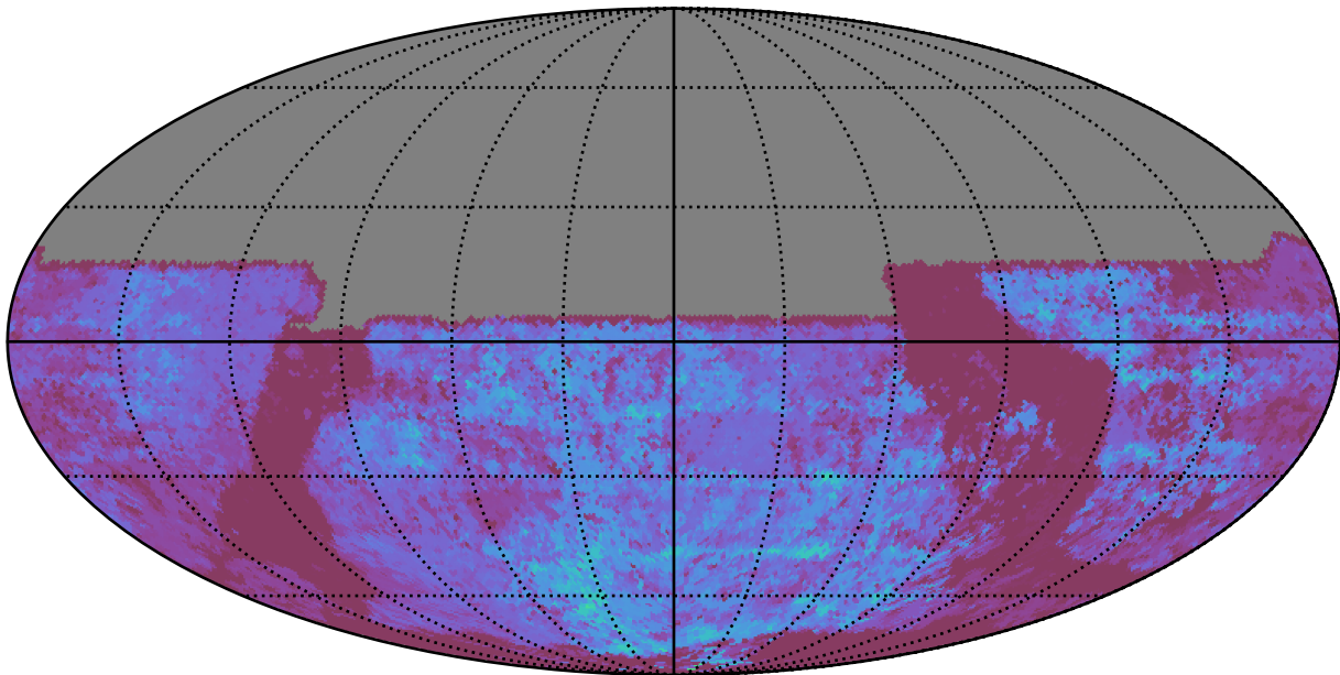
ddf_acor_sf30_lsf40_lsr10_v3.4_10yrs All sky u band: Median Season Length
