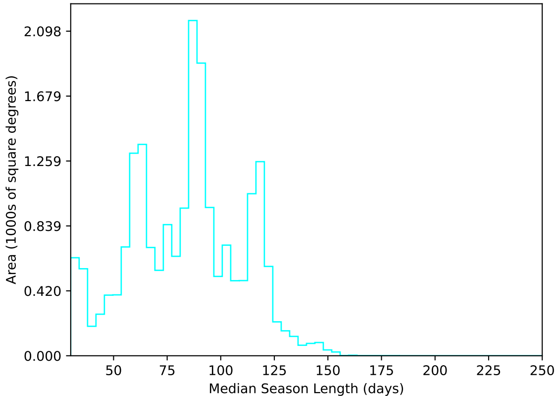
ddf_acor_sf30_lsf40_lsr10_v3.4_10yrs All sky u band: Median Season Length
