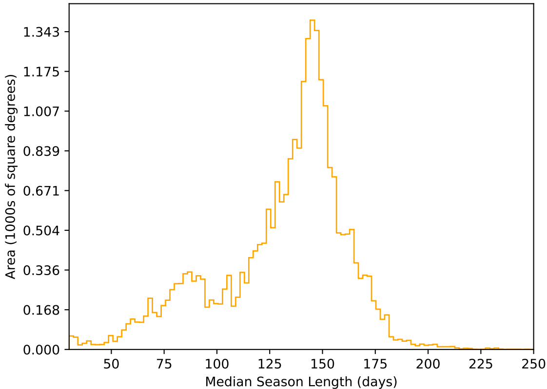
ddf_acor_sf30_lsf40_lsr10_v3.4_10yrs All sky r band: Median Season Length
