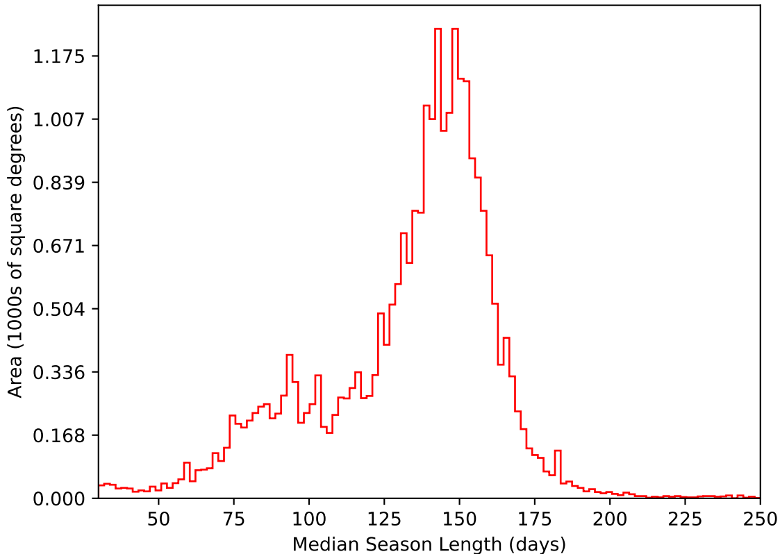
ddf_acor_sf30_Isf40_Isr10_v3.4_10yrs All sky i band: Median Season Length
