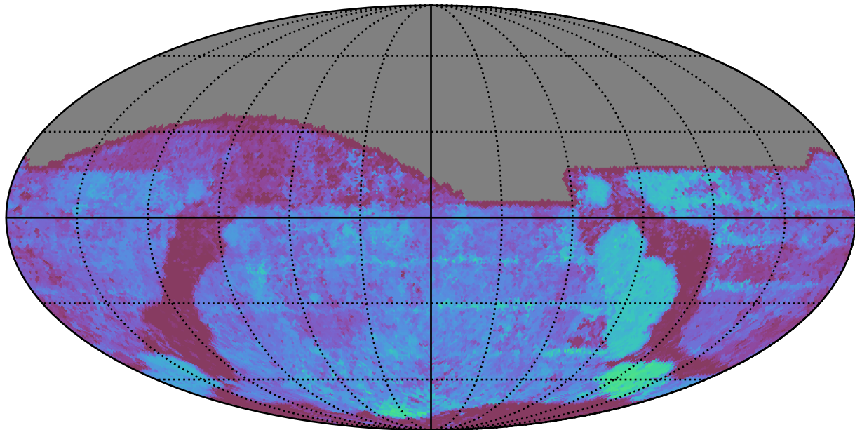
ddf_acor_sf30_lsf40_lsr10_v3.4_10yrs All sky g band: Median Season Length
