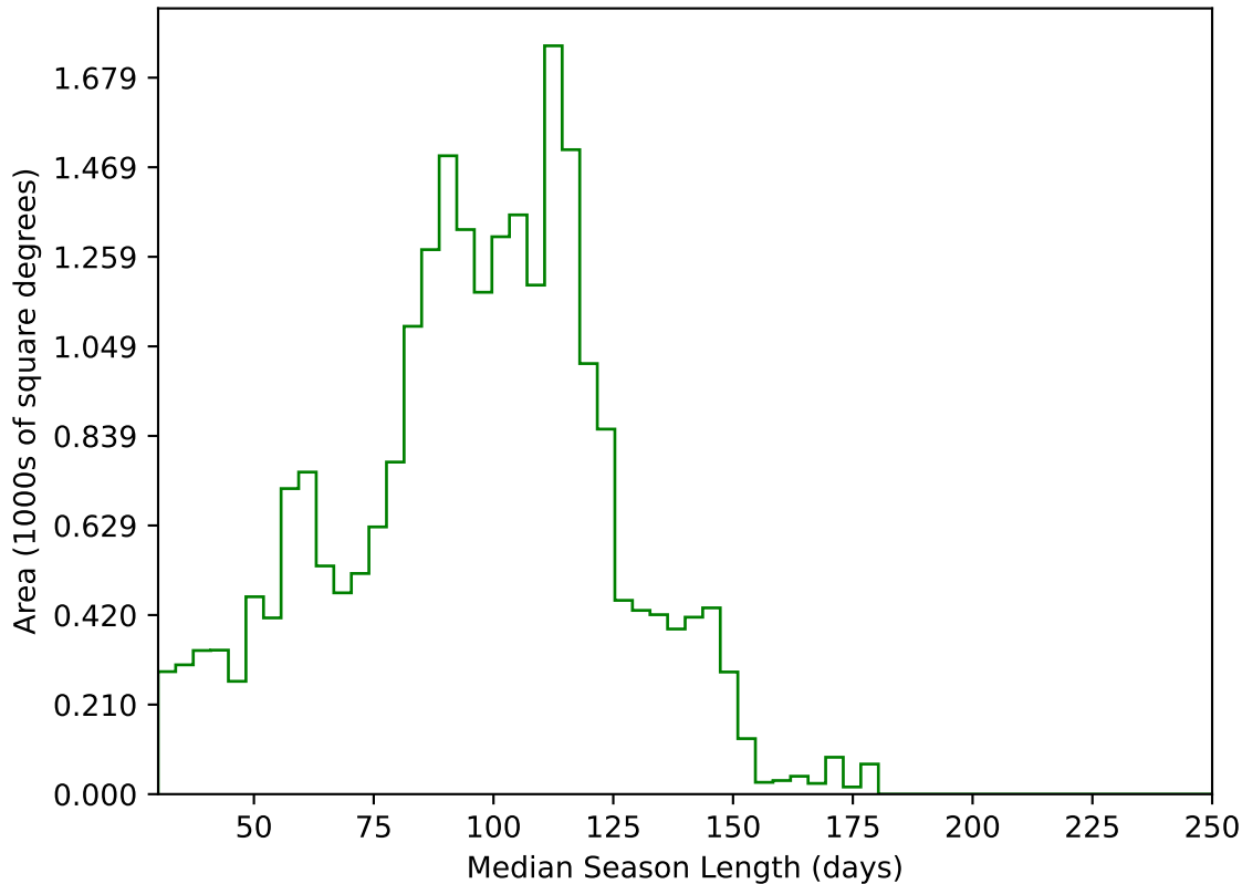
ddf_acor_sf30_lsf40_lsr10_v3.4_10yrs All sky g band: Median Season Length
