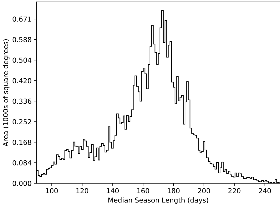
ddf_acor_sf30_lsf40_lsr10_v3.4_10yrs All sky all bands: Median Season Length
