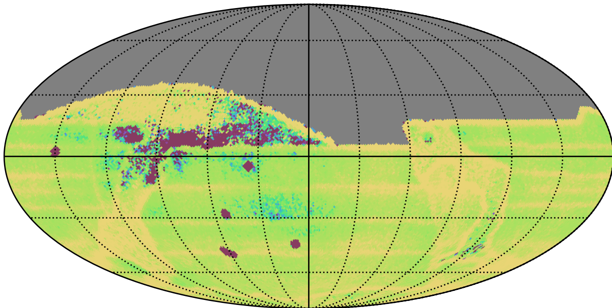
ddf_acor_sf30_lsf40_lsr10_v3.4_10yrs All sky: Median Intra-Night Gap
