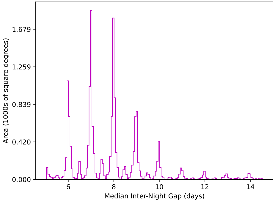
ddf_acor_sf30_lsf40_lsr10_v3.4_10yrs WFD z band: Median Inter-Night Gap
