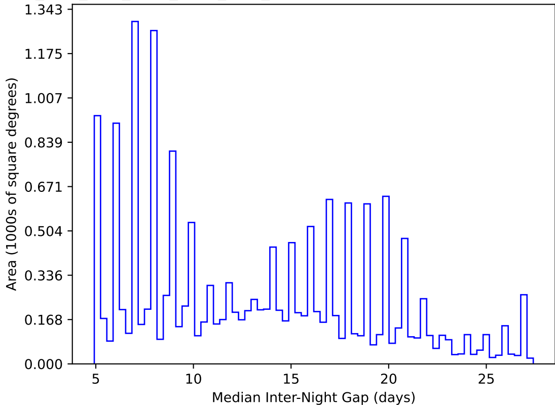
ddf_acor_sf30_lsf40_lsr10_v3.4_10yrs WFD y band: Median Inter-Night Gap
