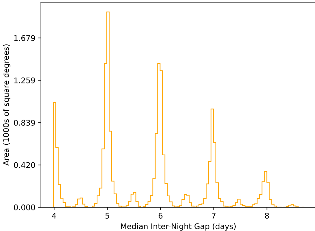
ddf_acor_sf30_lsf40_lsr10_v3.4_10yrs WFD r band: Median Inter-Night Gap
