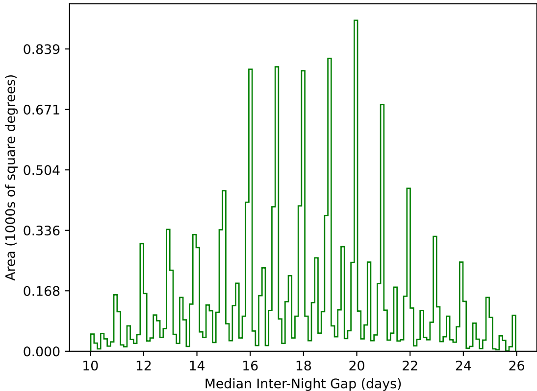
ddf_acor_sf30_lsf40_lsr10_v3.4_10yrs WFD g band: Median Inter-Night Gap
