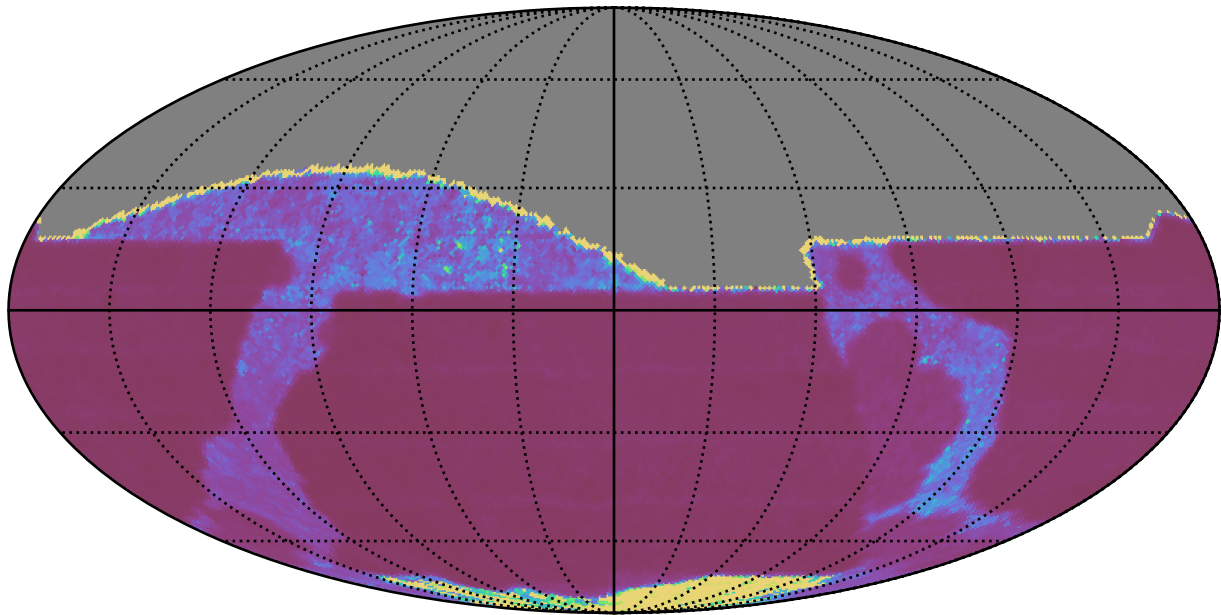
ddf_acor_sf30_lsf40_lsr10_v3.4_10yrs All sky z band: Median Inter-Night Gap
