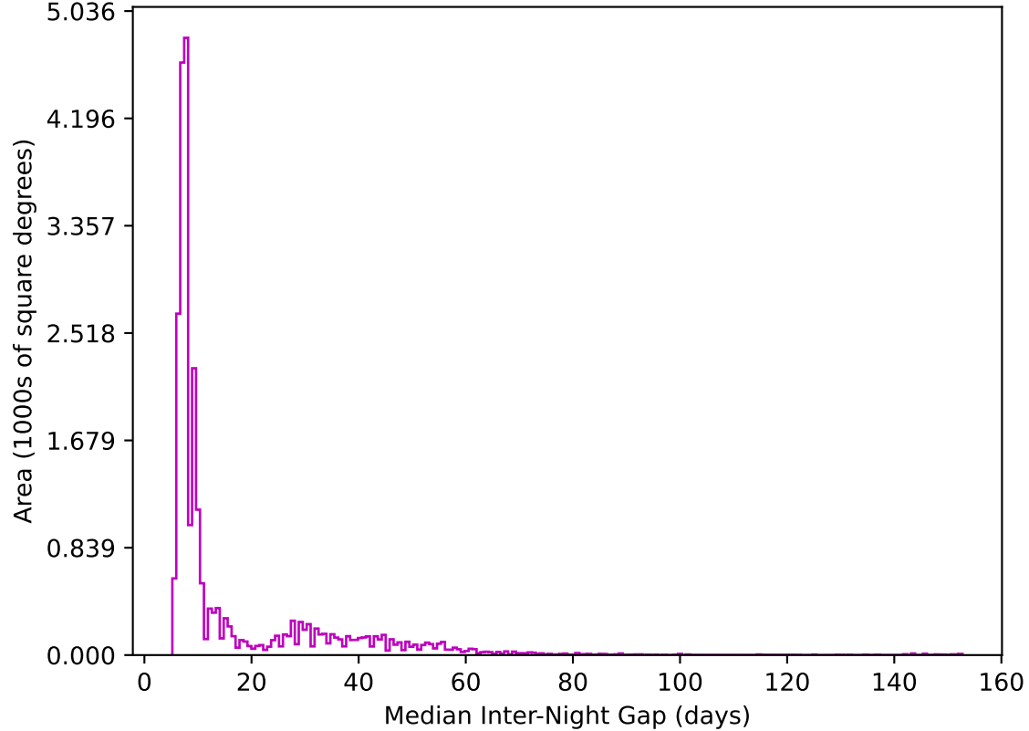
ddf_acor_sf30_lsf40_lsr10_v3.4_10yrs All sky z band: Median Inter-Night Gap
