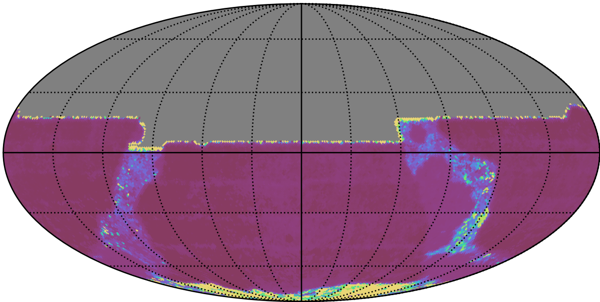
ddf_acor_sf30_lsf40_lsr10_v3.4_10yrs All sky y band: Median Inter-Night Gap
