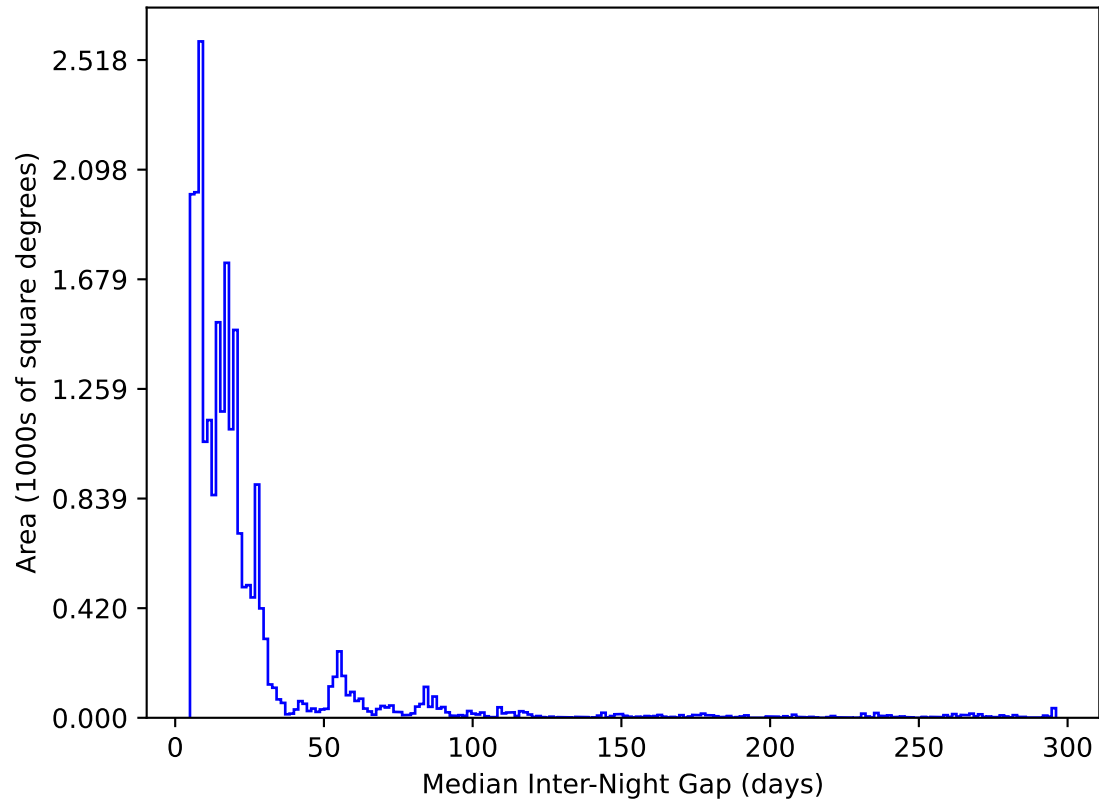
ddf_acor_sf30_lsf40_lsr10_v3.4_10yrs All sky y band: Median Inter-Night Gap
