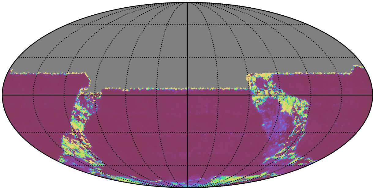
ddf_acor_sf30_lsf40_lsr10_v3.4_10yrs All sky u band: Median Inter-Night Gap
