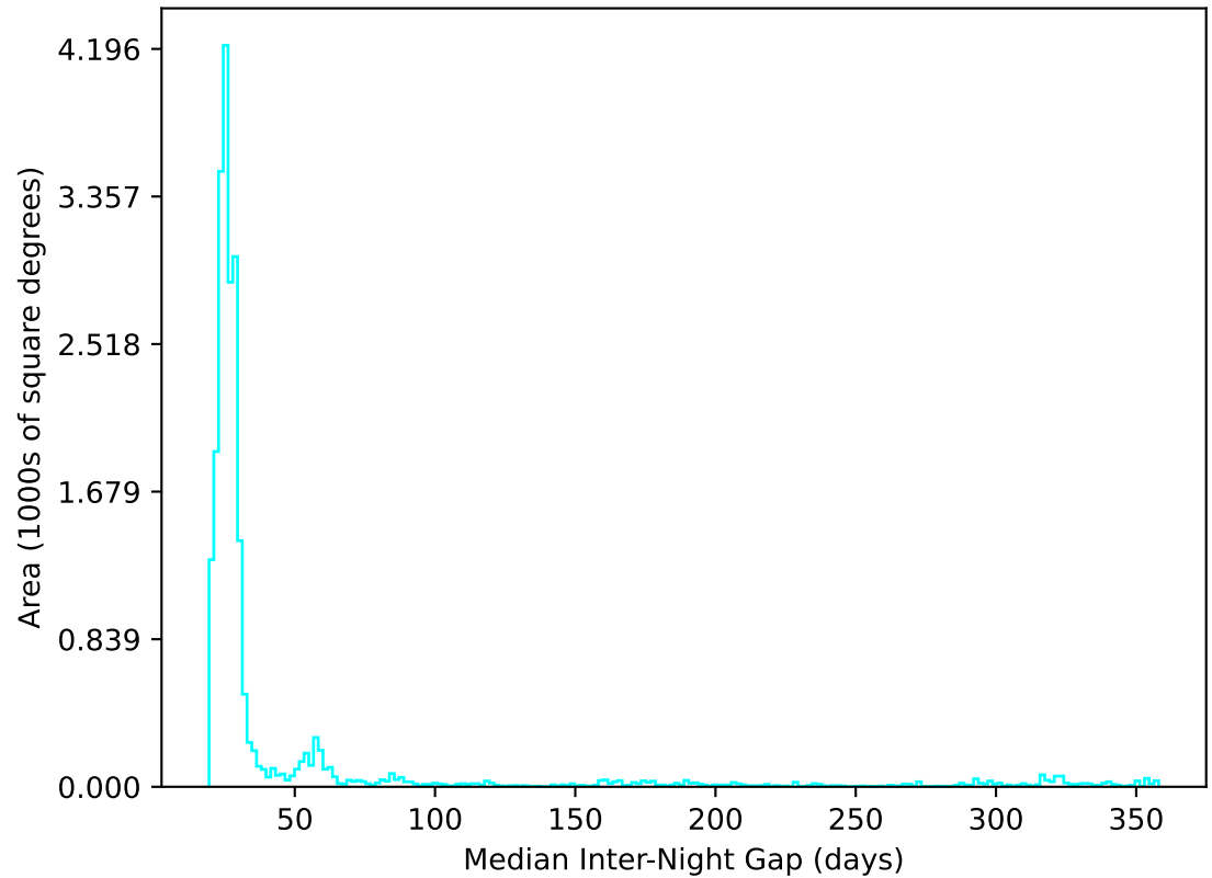
ddf_acor_sf30_lsf40_lsr10_v3.4_10yrs All sky u band: Median Inter-Night Gap
